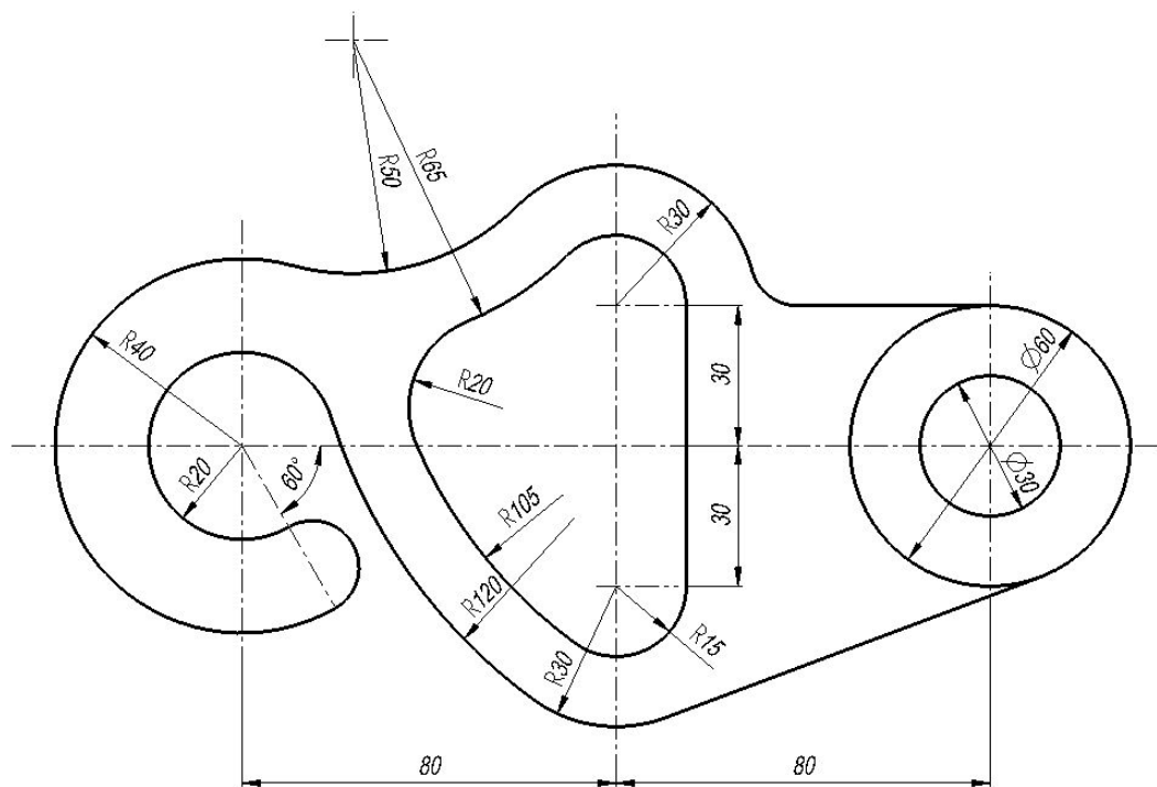
Prob.3-11. Locking Device
