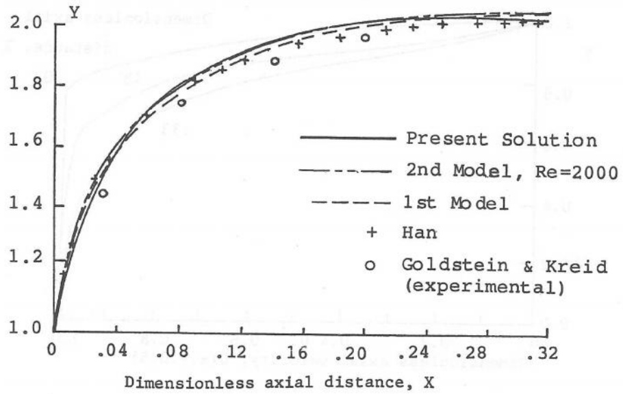
Figure 5 Axial velocity development at duct center line
