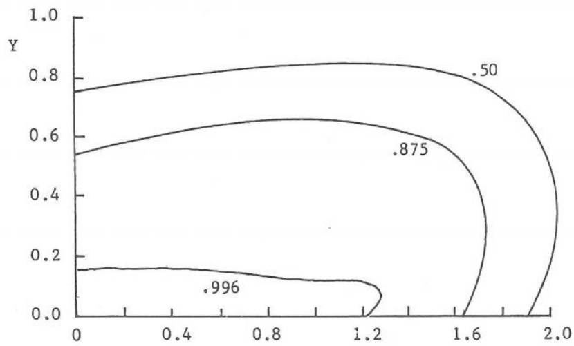
Figure 10 Axial velocity profiles on Y - Z plane at X = 0.3
