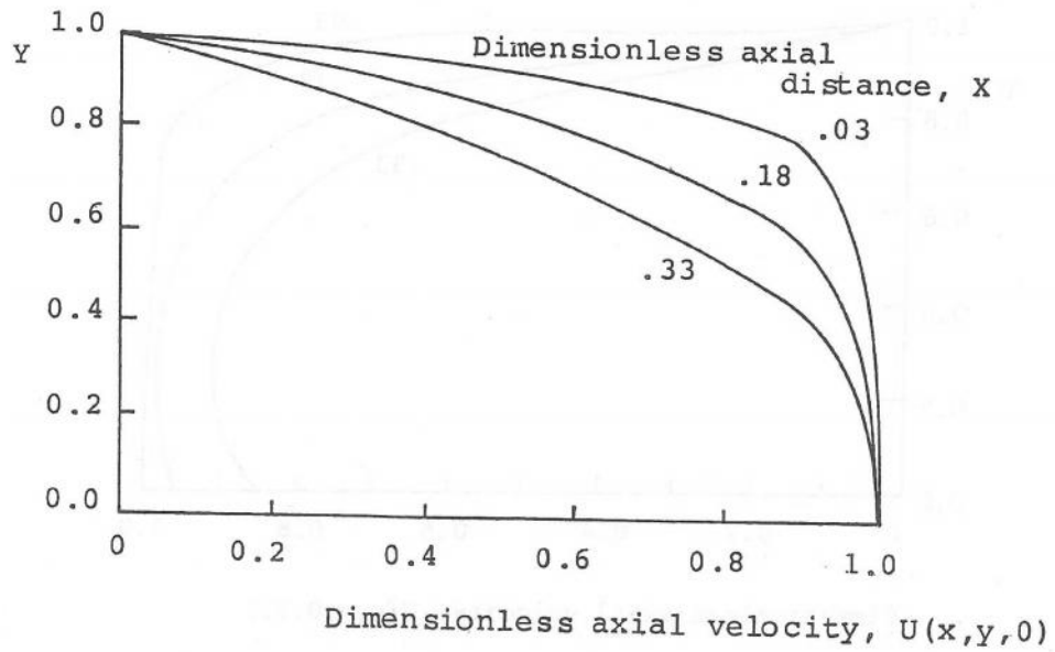
Figure 6 Axial velocity profiles on center plane Z = 0
