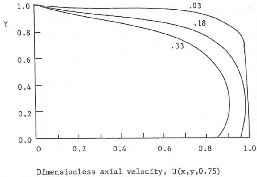
Figure 8 Axial velocity profiles on the plane Z = 0.75
