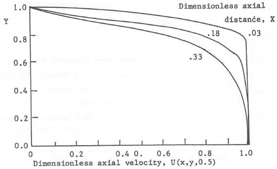
Figure 7 Axial velocity profiles on the plane Z = 0.5
