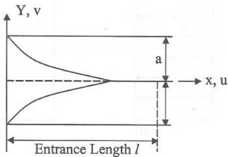
Figure 2 Physical model of entrance region in X-Y plane
