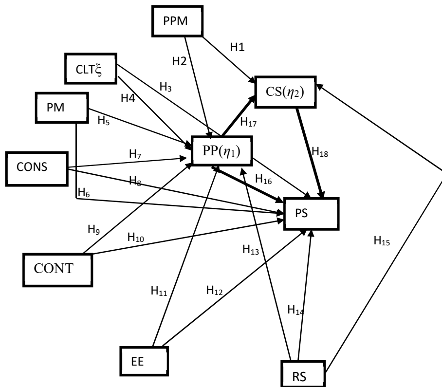
Figure 1: Hypothetical model for SEM
