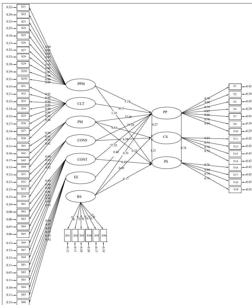
Figure 7: Modified SEM model
